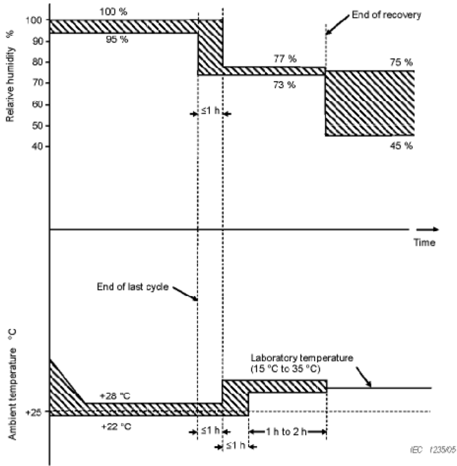
Figure 3 – Test Db – Recovery at controlled conditions
