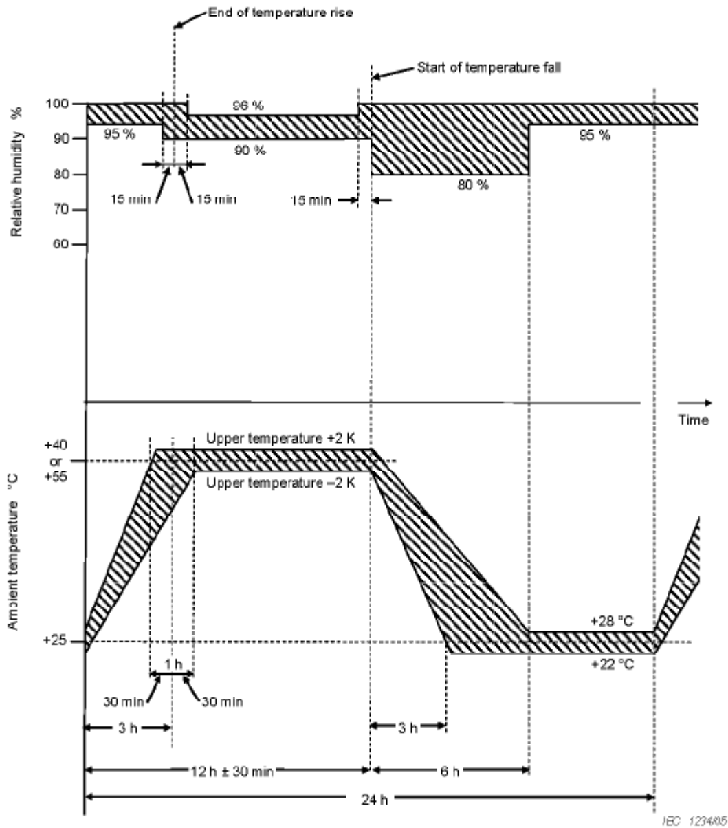
Figure 2b – Test Db – Test cycle – Variant 2
