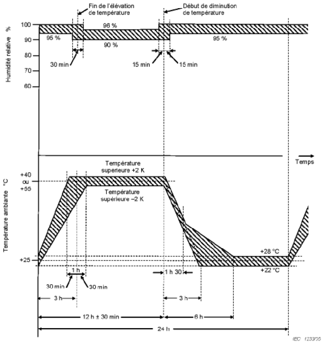
Figure 2a – Essai Db – Cycle d'essai – Variante 1
