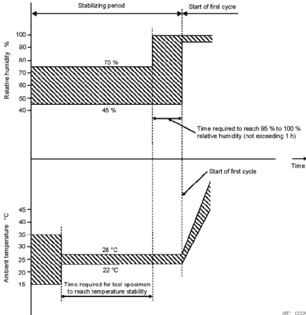
Figure 1 – Test Db – Stabilizing period
